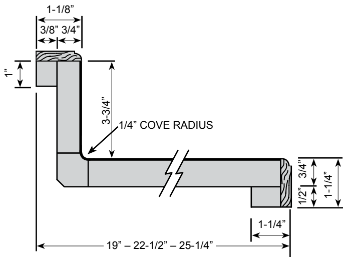
KITCHEN & VANITY TOP
